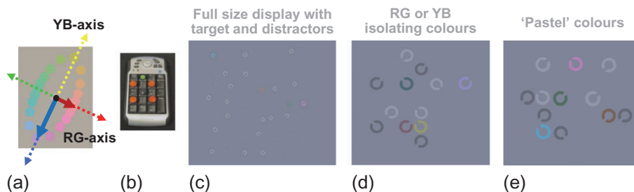
Fig. 15 Examples of visual search experiments involving coloured stimuli ( c ) and magnified regions to show the use of isolating RG and YB colours ( d ) and ‘pastel’ colours ( e ). The latter stimulate both the RG and the YB chromatic mechanisms and are therefore perceived to have some colour even by protanopes and deuteranopes. 3 The YB and RG colour isolating axes with respect to a D_{65} background are shown in ( a ) and the subject’s response keypad in ( b ).
