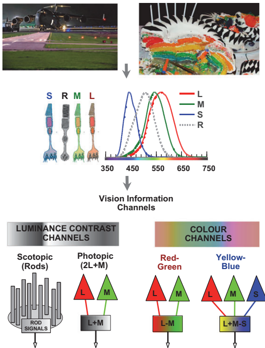
Fig. 1 Typical scenes where colour is useful, important and attractive. Information in complex scenes is extracted and channelled to the cortex efficiently via four principal ‘vision information’ channels. There are two achromatic channels which detect spatial differences in the amount of light in the retinal image over a large range of ambient illumination. These are often described as the ‘photopic’ and the ‘scotopic’ luminance channels. The photopic channel relies on the sum of L- and M-cone signals and carries no colour information. The scotopic channel relies on spatially pooled rod signals to achieve high sensitivity to light at the expense of spatial resolution. RG colour discrimination relies on differences in the amount of long-wavelength and middle-wavelength light as detected by L and M cones. S-cone signals reflect the amount of short-wavelength light present at a given point in the retinal image. Comparison of S-cone signals with the signals generated in L and M cones forms the basis for the YB channel. The signals generated in these two colour channels operate selectively through distinct mechanisms in the retina, but are then combined in later stages, when suprathreshold colour processing is involved, to yield the many colours we see.
