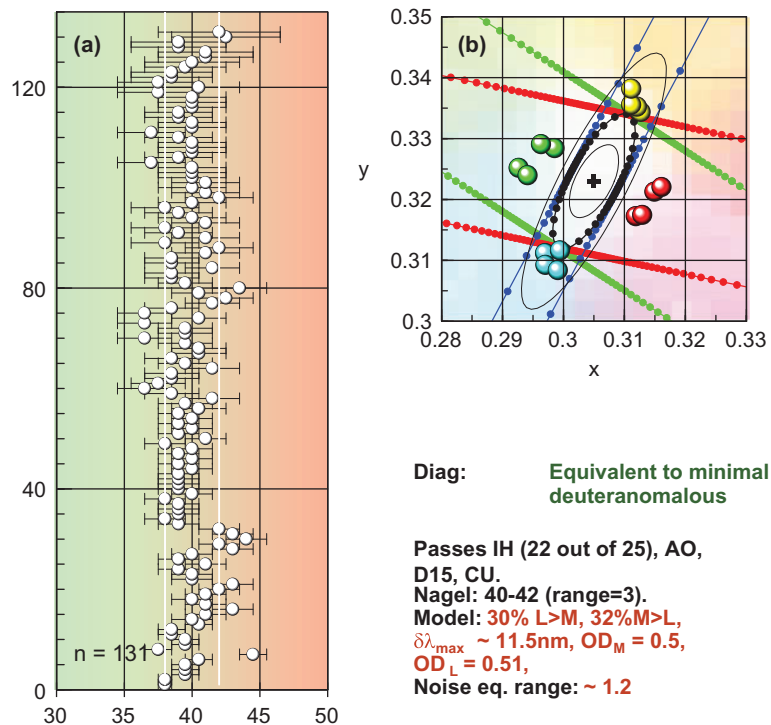
Fig. 13 The midpoints measured in normal trichromats and ranked in increasing matching range in (a) are the same as those plotted in Figure 11a, but on a magnified scale that shows the large variability which exists in normal trichromats. More importantly, the very few subjects that may rely on two variant genes make completely normal anomaloscope matches but exhibit slight loss of RG chromatic sensitivity, typical of the least affected deuteranopes. The subject shown in (b) makes completely normal Nagel anomaloscope matches (with a midpoint of 41 and a range of 3 units). The subject also passes D15, AO HRR and City University (2nd Ed.) CV tests and makes only two errors on the IH-38 plates edition.
