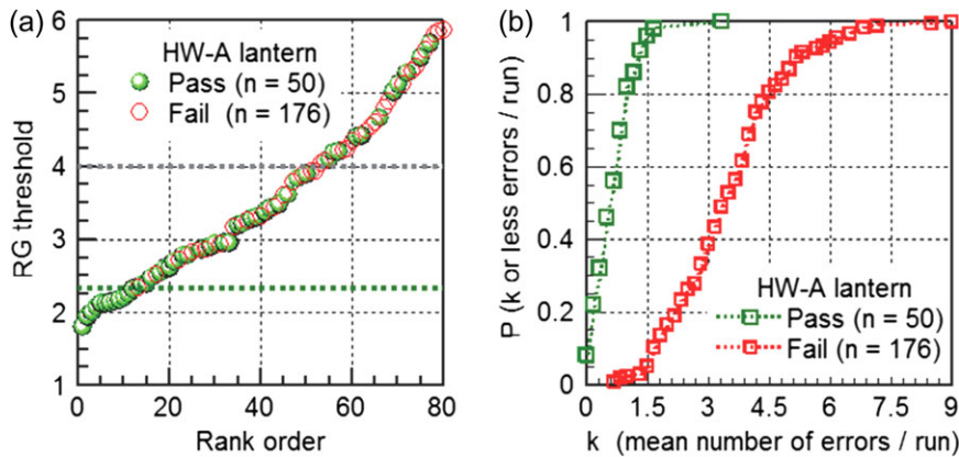
Fig. 11 Ranked distribution of CAD RG thresholds for the 226 deutan subjects (a) investigated. (b) A plot of the probability of making, k , or fewer errors per run for the deutan subjects that pass and for those that fail the HW-A protocol. Each subject carried out a total of 6 tests (i.e. 54 presentations of the paired vertical lights).
