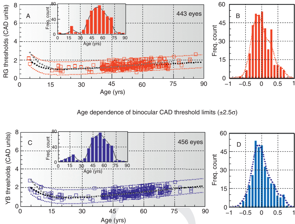
Figure 8.7 RG (panels A and B) and YB (panels C and D) binocular thresholds as a function of age for all the subjects examined in the study and deemed to have normal color vision. Conversion from monocular to binocular thresholds was carried out by using the mean monocular to binocular ratio measured in 57 subjects with normal color vision. Best eye monocular to binocular ratios were calculated with means ( \mu ) and standard deviations ( \sigma ) of 1.29 and 0.16 for RG and 1.3 and 0.18 for YB color vision, respectively. The ratios of right and left eye thresholds were 1.03 (RG) and 1.02 (YB), neither being significantly different from unity. The histograms (panels B and D) plot the differences between the measured RG and YB thresholds (in CAD units) and the corresponding mean values derived from the best-fit functions (black, dotted lines).
