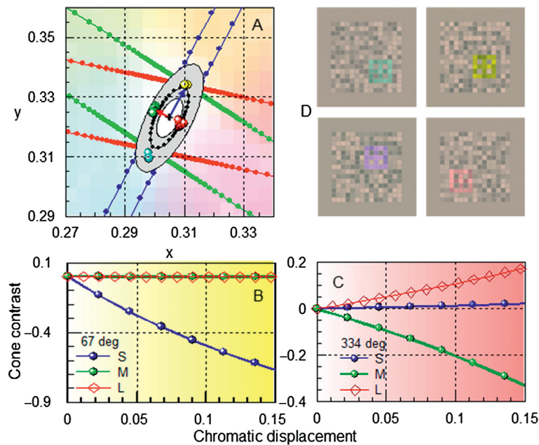
Figure 8.1 The statistical limits for the standard normal (SN) CAD observer (Barbur et al. , 2006; Rodriguez-Carmona, Harlow, Walker, and Barbur, 2005) are plotted in the CIE ( x,y ) 1931 chromaticity chart ( panel A ). The black cross at the center of the diagram shows the chromaticity of the white background; that is, 0.305, 0.323. The dotted black ellipse represents the median values computed from the distribution of RG and YB thresholds in 333 normal trichromats. The red and blue arrows indicate the corresponding SN unit for RG and YB color vision, respectively. The gray-shaded area represents the statistical distribution of thresholds shown in Figure 8.2B and C. The inner and outer ellipses represent the 2.5% and the 97.5% limits of variability, respectively. The red, green, and blue dotted lines denote the “color confusion bands” based on data measured in protanopes, deuteranopes, and tritanopes, respectively. The large colored dots within the center gray area plot measured thresholds typical of a normal trichromat. The corresponding cone contrasts for chromatic displacement (CD) along the YB ( 67^\circ ) and RG ( 334^\circ ) directions are shown in panels B and C, respectively. The maximum CD distances shown correspond to \sim 14 SN thresholds units for YB discrimination and \sim 34 SN units for RG discrimination. The non-linearity increases with the size of CD involved, particularly for the YB axis, but the departure from linearity is small for both RG and YB thresholds, even for CD values that are well above threshold. The screen dumps in panel D show the RG and YB stimuli employed in the CAD test.
